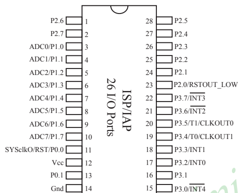
SOP-28/SKDIP-28
