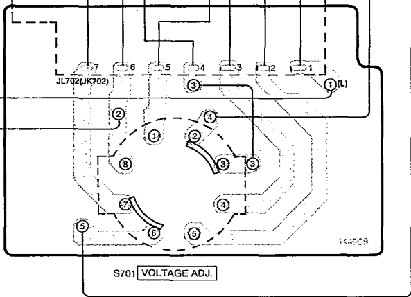
F VOLTAGE SELECTOR P.C.B. (REP2152B-P)
