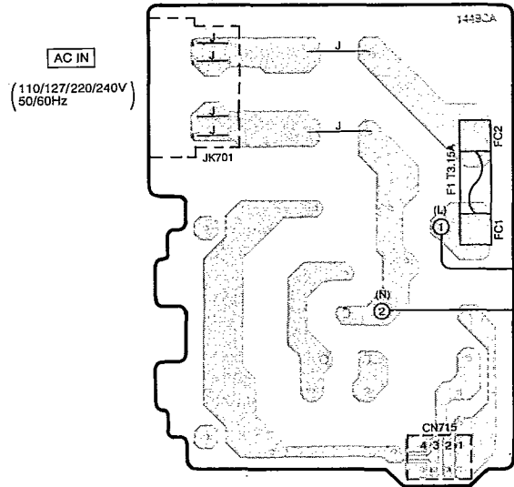
E AC IN TERMINAL P.C.B. (REP2152B-P)
