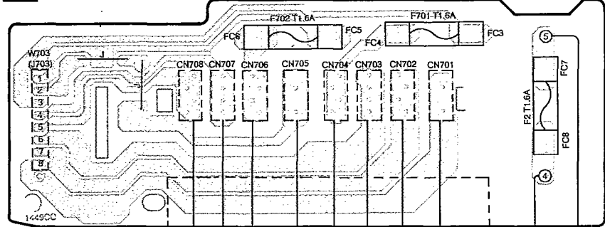
D POWER TRANSFORMER P.C.B. (REP2152B-P)
