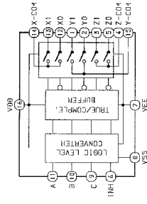
IC, TC4053BP
