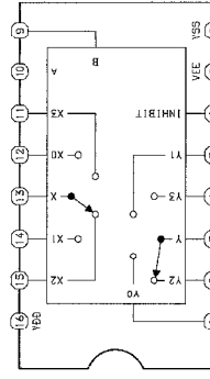
IC, TC4052EP
