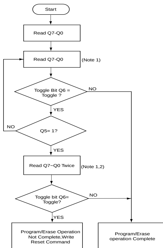
FIGURE 19. TOGGLE BIT ALGORITHM
