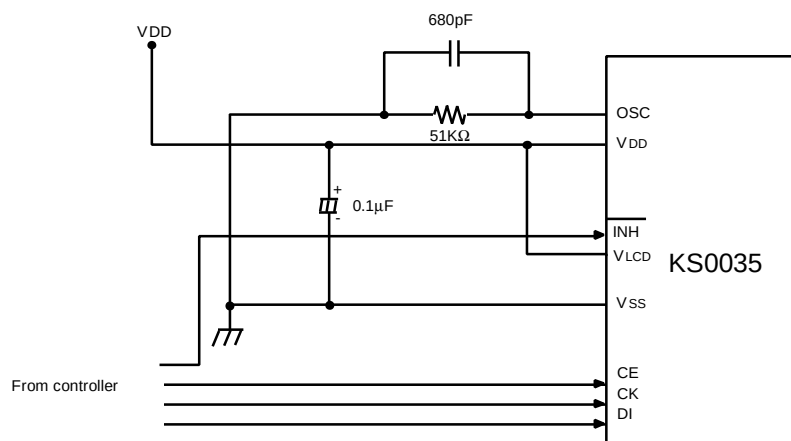
Application circuit 2
