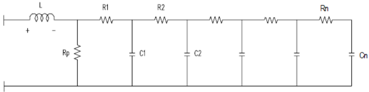
Figure 5: Ladder Network
