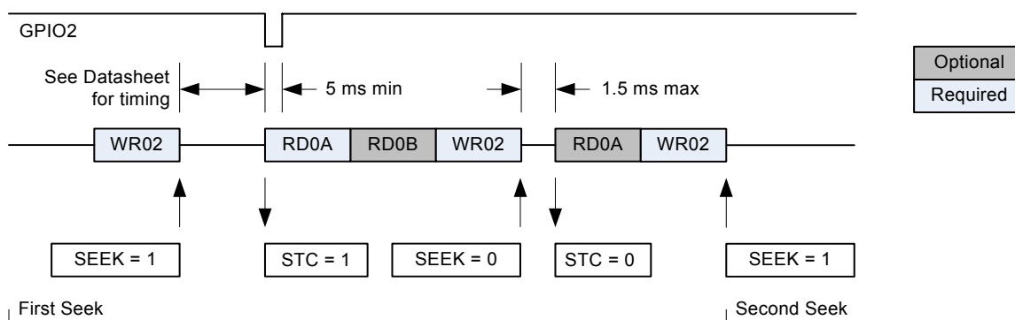
Figure 11. Seek Timing
