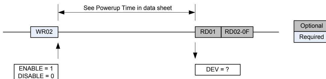
Figure 8. Powerup Timing
