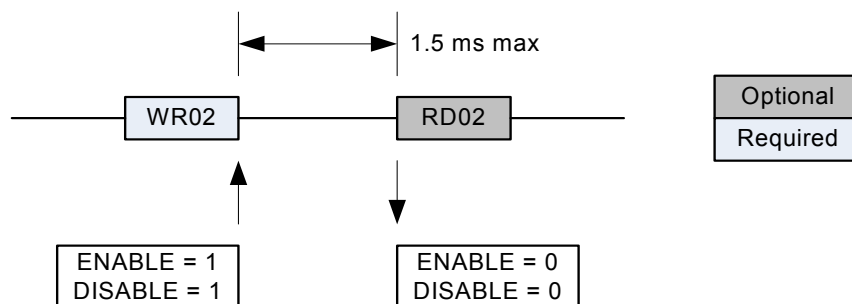
Figure 9. Powerdown Timing
