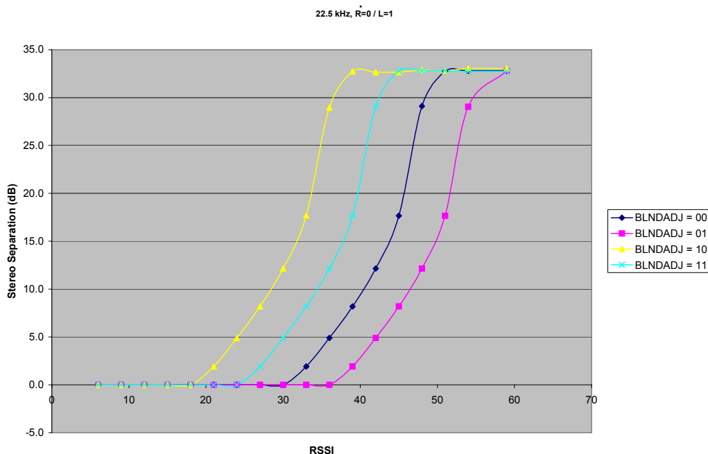
Figure 10. Stereo Separation
