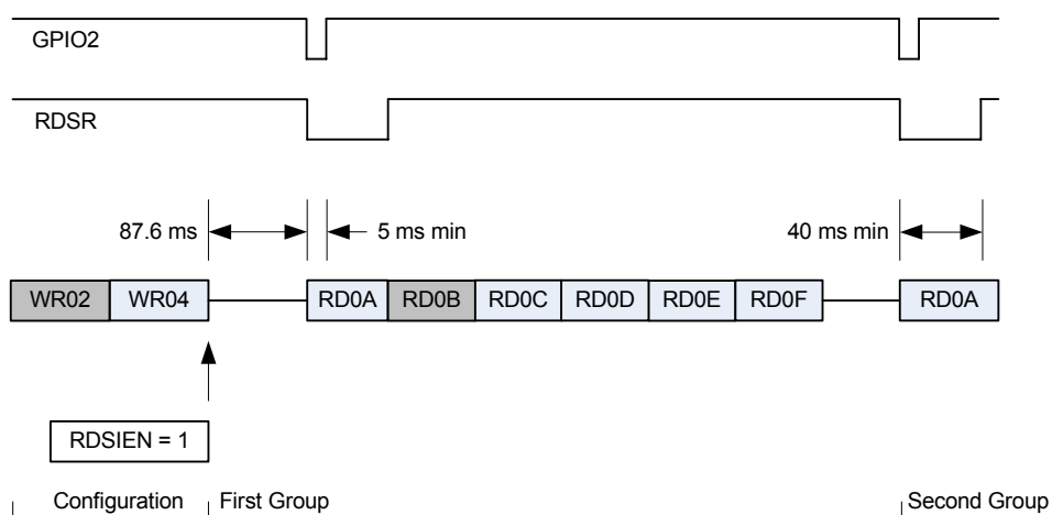
Figure 15. RDS Timing
