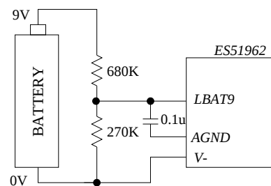
(e) Testing battery-low function.
