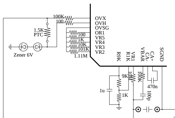
21 (g) Testing capacitance measurement. July 5, 2002
