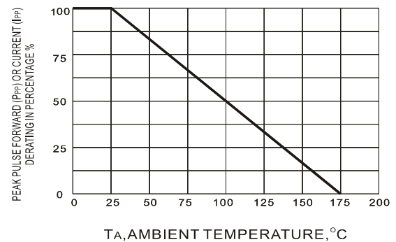
Fig.2 PULSE DERATING CURVE
