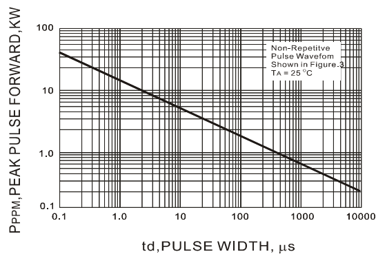
Fig.1 PEAK PULSE POWER RATING PULSE TIME CURVE
