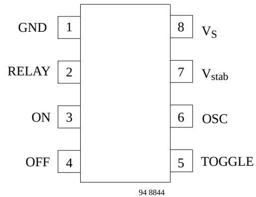
Figure 2. Pinning
