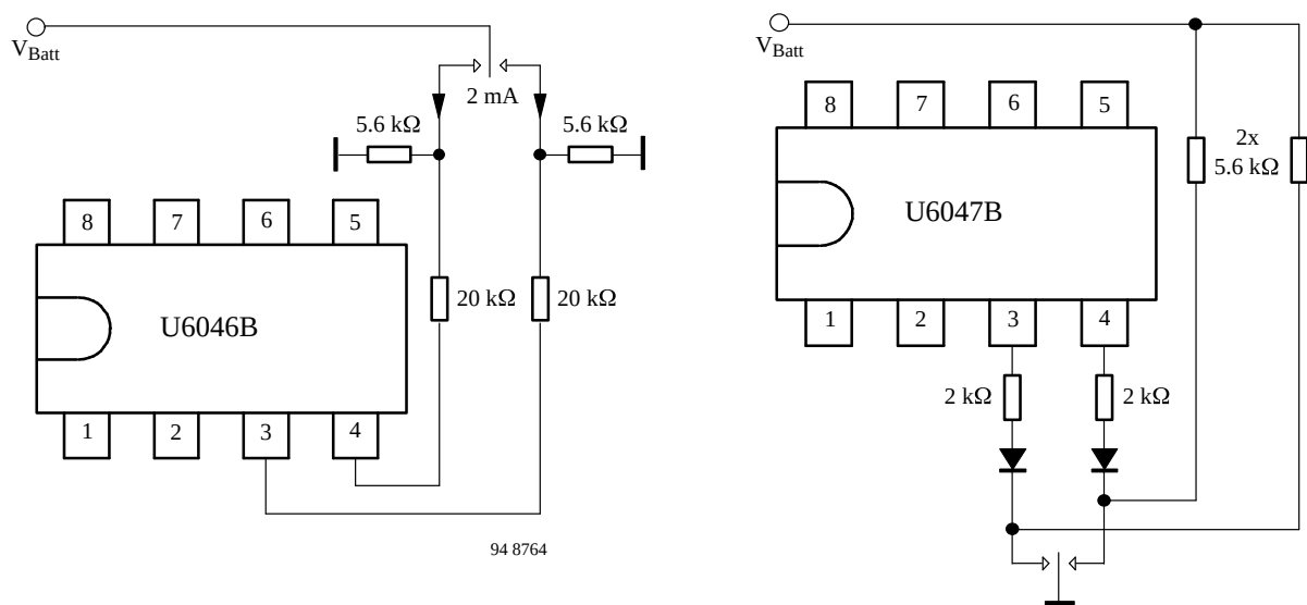
Figure 15. Increasing the contact current by parallel resistors
