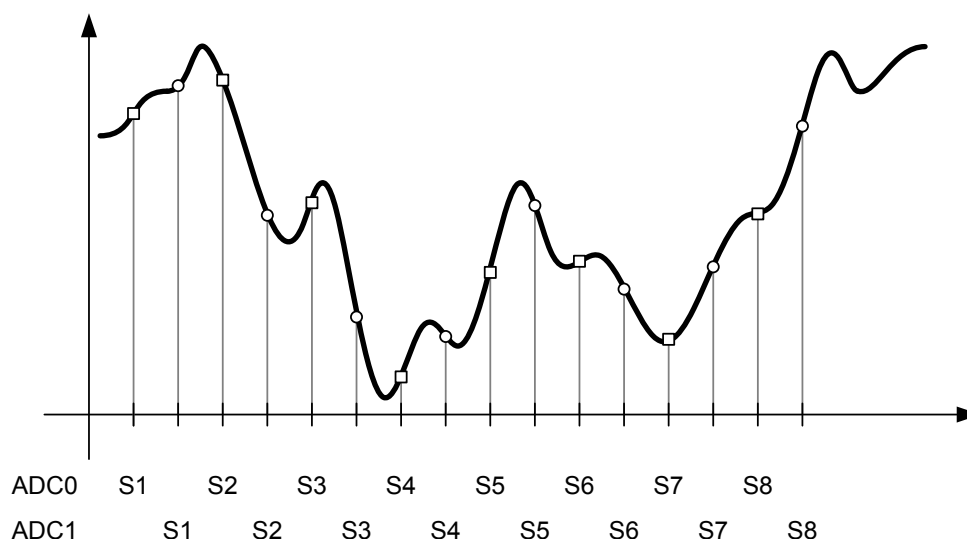
Figure 14-5. Skewed Sampling
