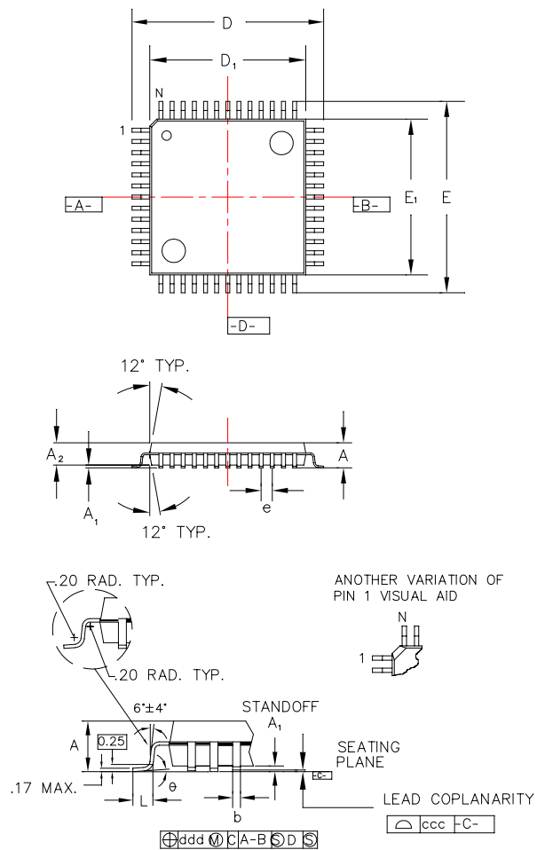
Figure C-1. 100-Pin LQFP Package
