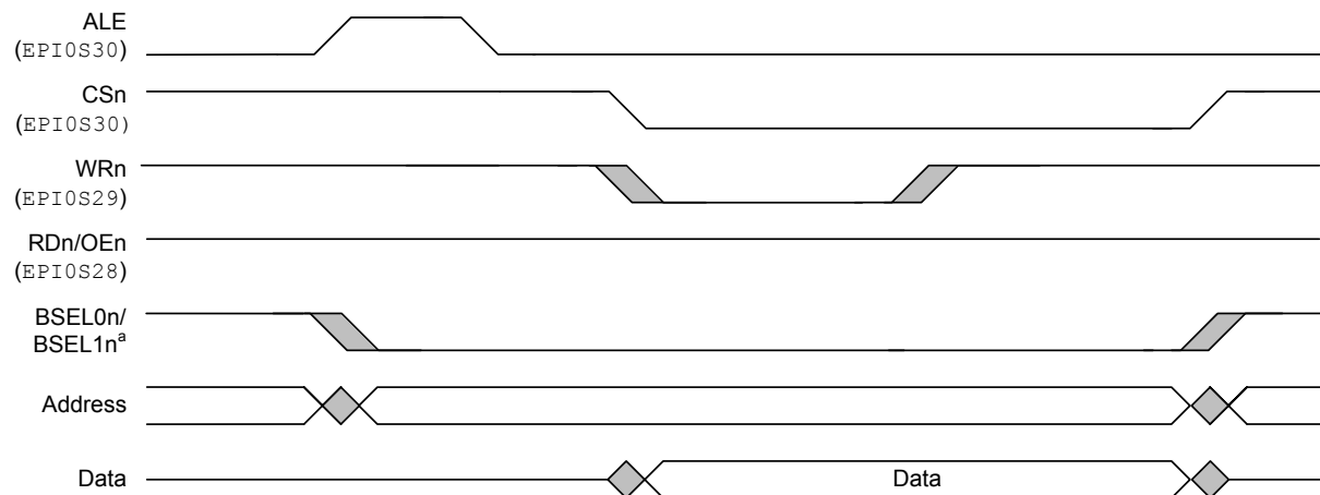
Figure 11-6. Host-Bus Write Cycle, MODE = 0x1, WRHIGH = 1, RDHIGH = 1
