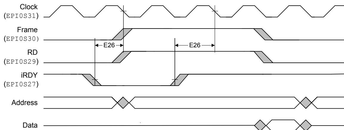
Figure 26-18. General-Purpose Mode iRDY Timing
