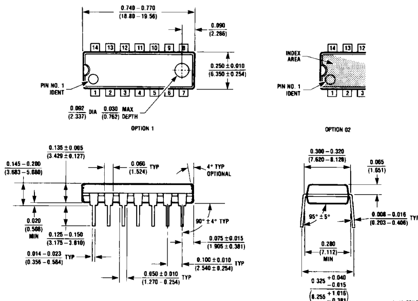
Molded Dual-In-Line Package (N) Order Number NM95C12N, NM95C12EN or NM95C12MN NS Package Number N14A
