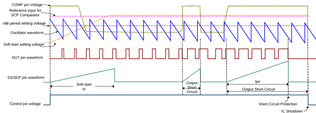
Figure 18. FP5139A Timing Diagram
