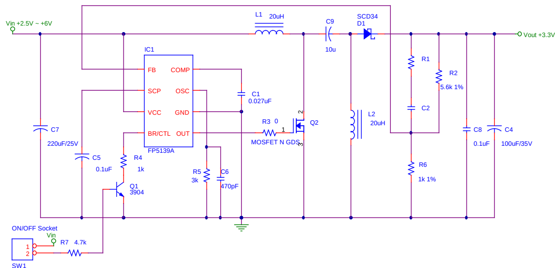
Figure 15. FP5139A DC2.5V~DC6V to DC3.3V SEPIC Regulator
