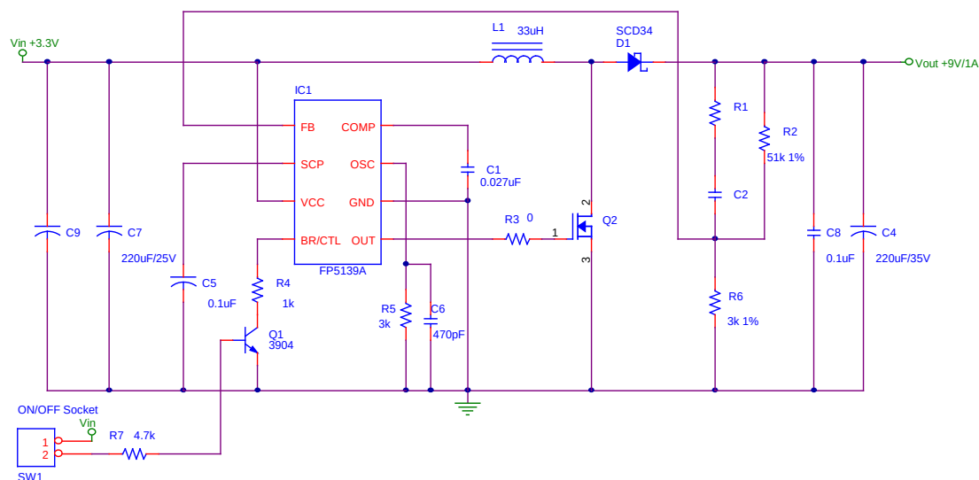
Figure 14. FP5139A DC3.3V to DC9V Boost Regulator
