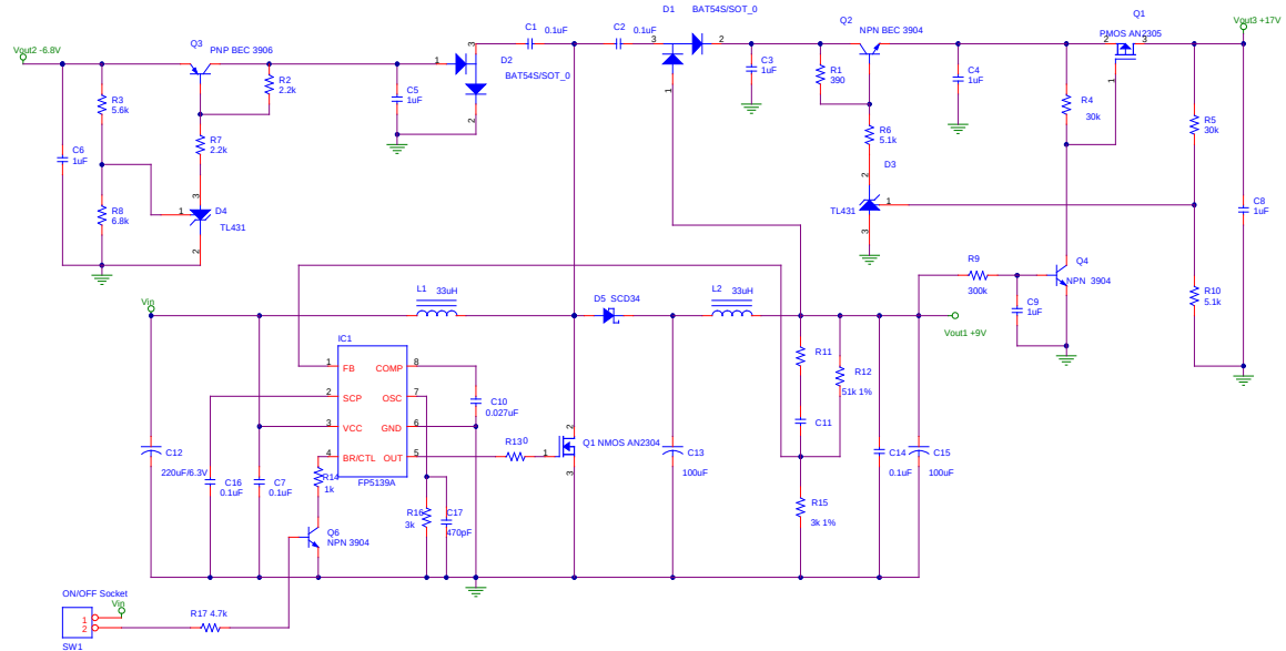
Figure 16. FP5139A Charge Pump DC-DC Converter Circuits
