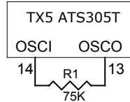
Oscillator Circuit
