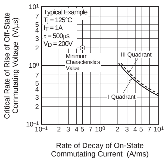
Commutation Characteristics
