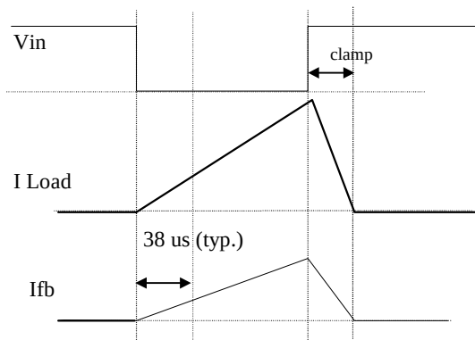
Figure 5 - Current sense precision: Accurate measurement only when the power Mosfet is fully ON
