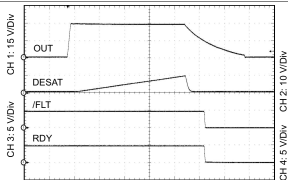
Figure 12. Output Transient Waveform DESAT, RDY and \overline{FLT}
