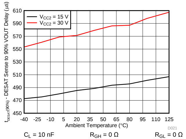
Figure 31. DESAT Sense to V_{OUT/HL} 90% Delay vs Temperature
