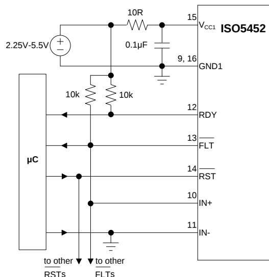
Figure 52. Global Shutdown with Inverting Input Configuration
