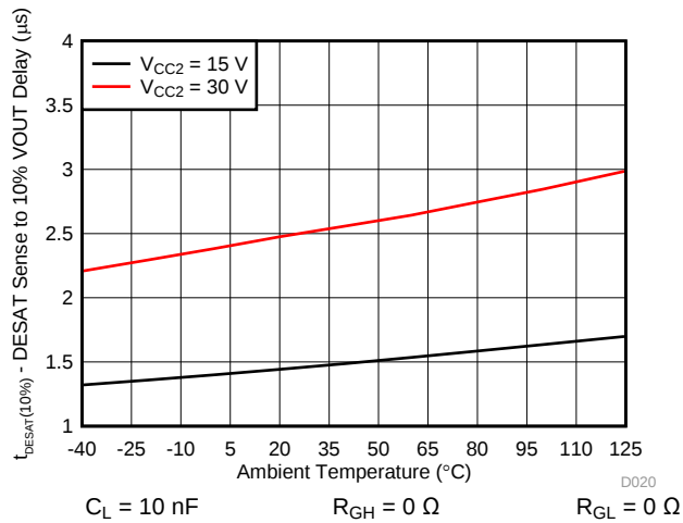
Figure 30. DESAT Sense to V_{OUT/HL} 10% Delay vs Temperature
