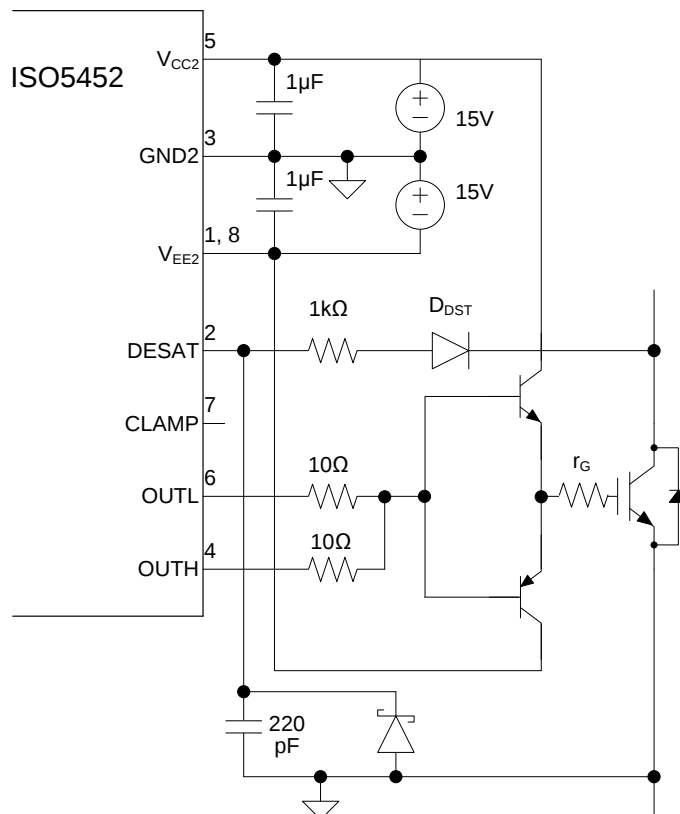
Figure 56. Current Buffer for Increased Drive Current
