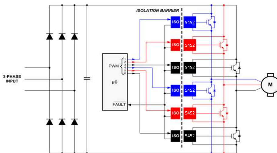
Figure 47. Typical Motor Drive Application
