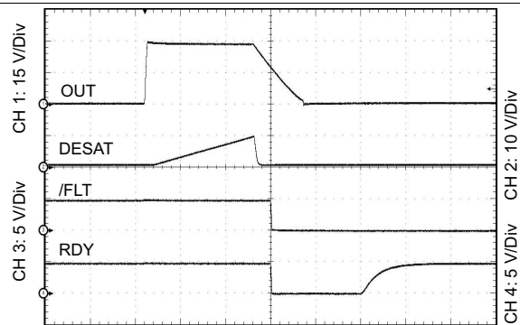
Figure 13. Output Transient Waveform DESAT, RDY and \overline{FLT}
