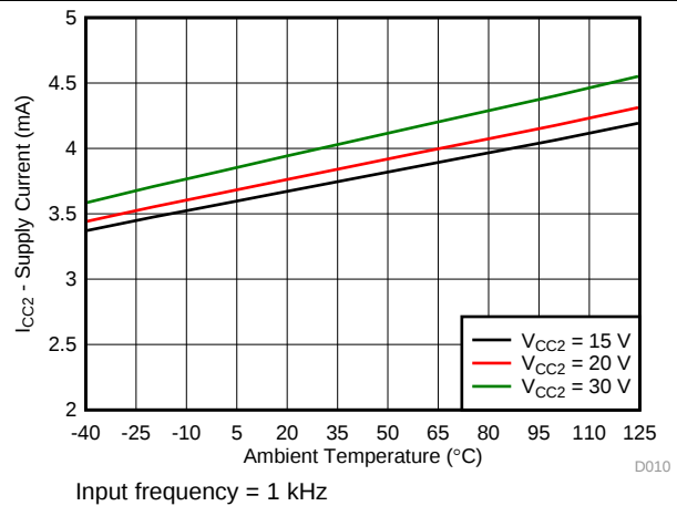
Figure 19. I_{CC2} Supply Current vs Temperature
