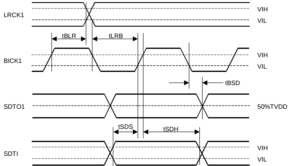
Audio Interface Timing (TDM0 = "1")
