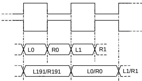
Figure 22. DAUX2 and VIN input timings
