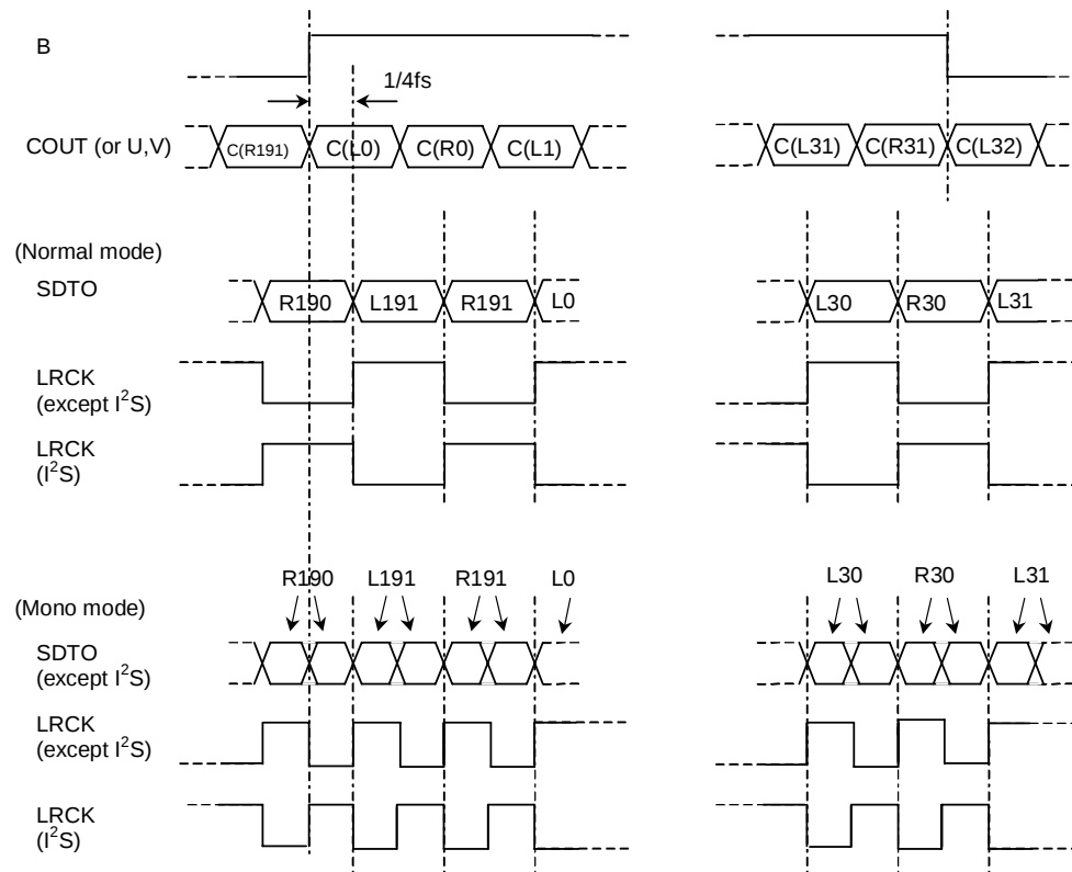
Figure 21. B, C, U, V output/input timings
