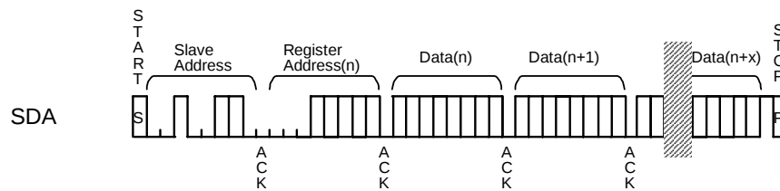
Figure 47. WRITE Operation
