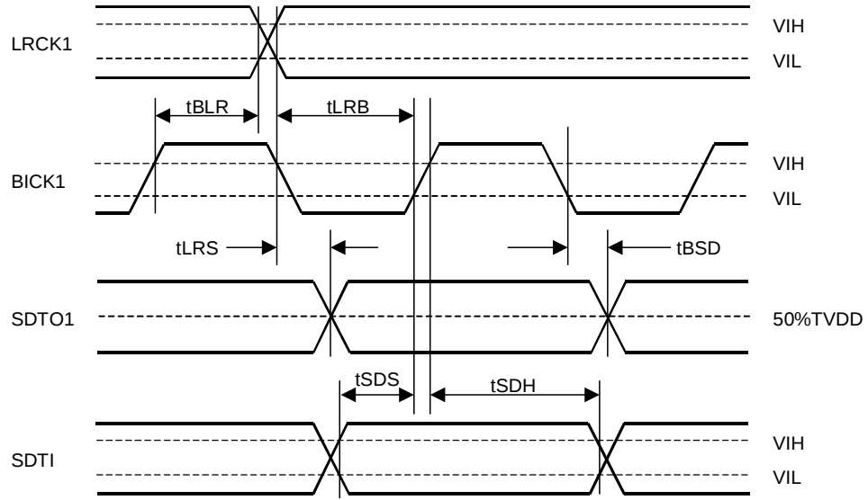
Audio Interface Timing (TDM0 = "0")
