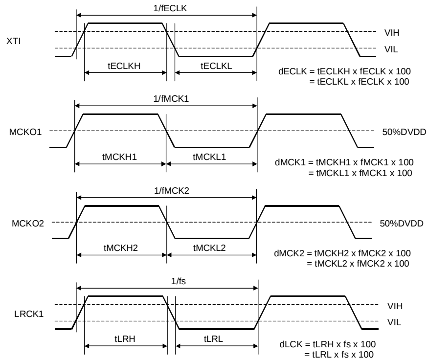
Clock Timing
