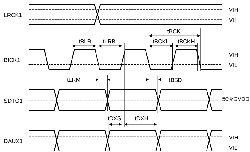
Clock Timing
