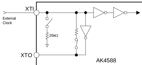
Figure 18. (a). External clock mode (Input : CMOS Level)
