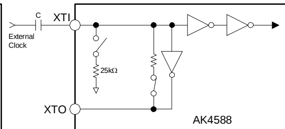
Figure 19. (b). External clock mode (Input : \geq 40\%DVDD )
