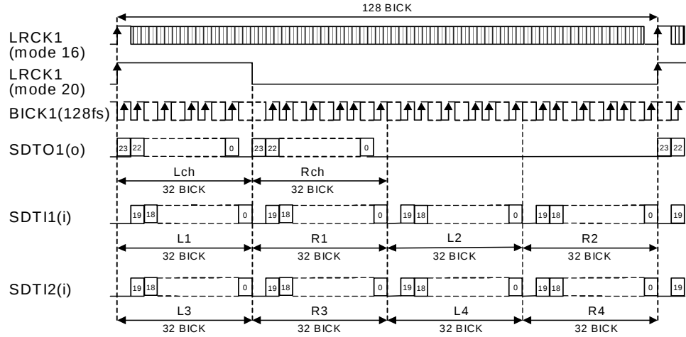
Figure 9. Mode 16,20 Timing
