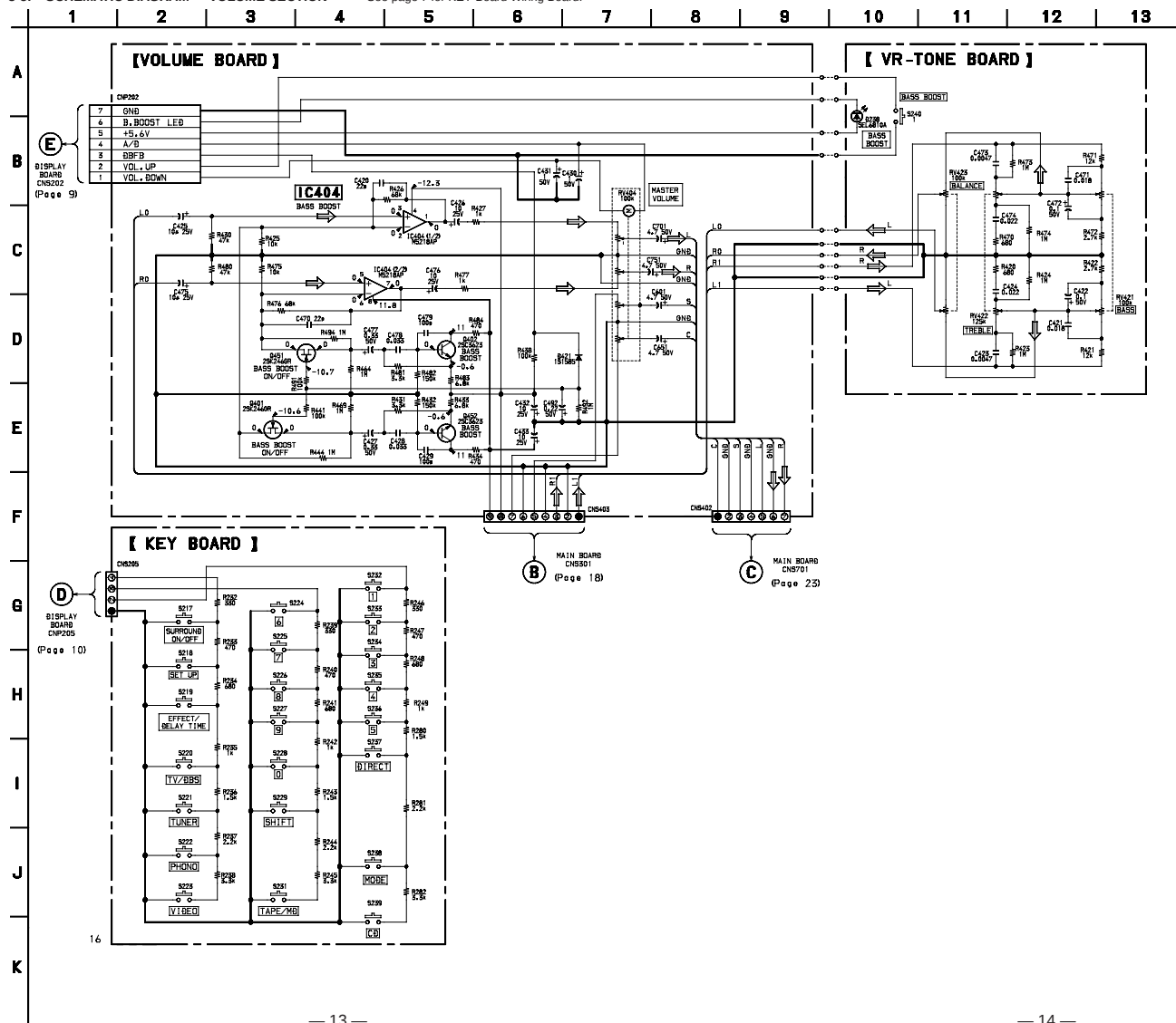
3-5. SCHEMATIC DIAGRAM — VOLUME SECTION — • See page 7 for KEY Board Wiring Board.
