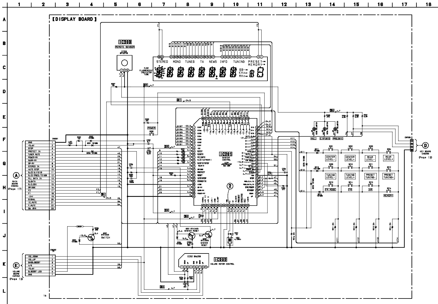
3-3. SCHEMATIC DIAGRAM — DISPLAY SECTION — • See page 6 for Waveforms. • See page 25 for IC Pin Functions. • See page 27 for IC Block Diagrams.
