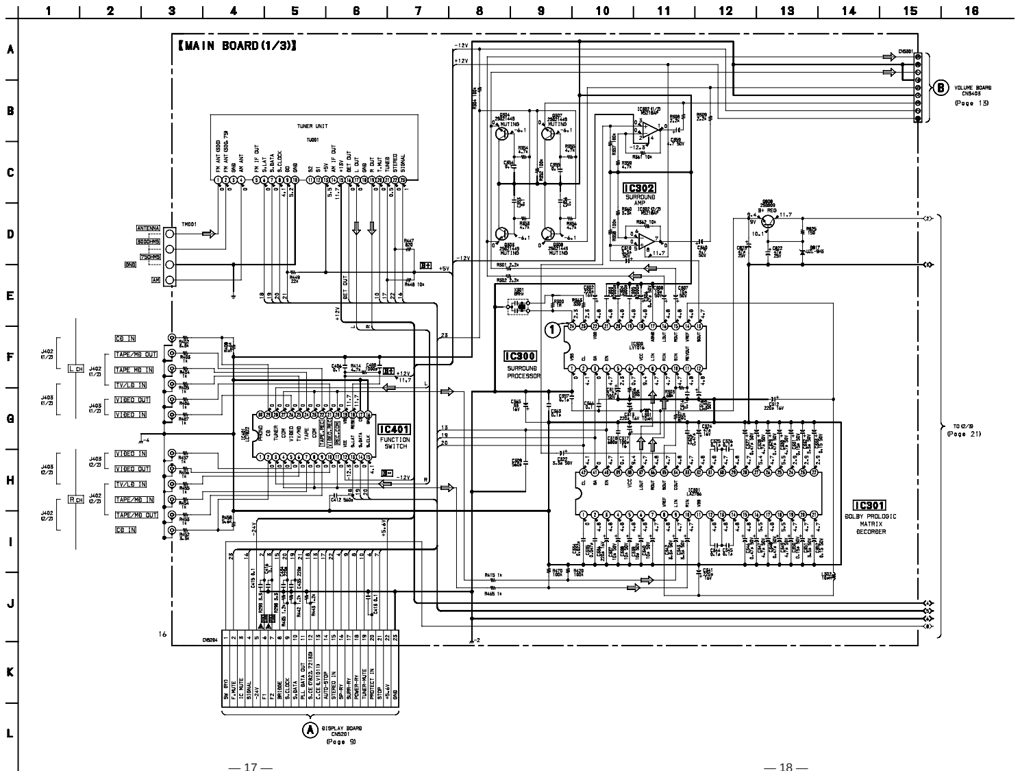
3-7. SCHEMATIC DIAGRAM — MAIN (1/3) SECTION — • See page 27 for IC Block Diagrams.
