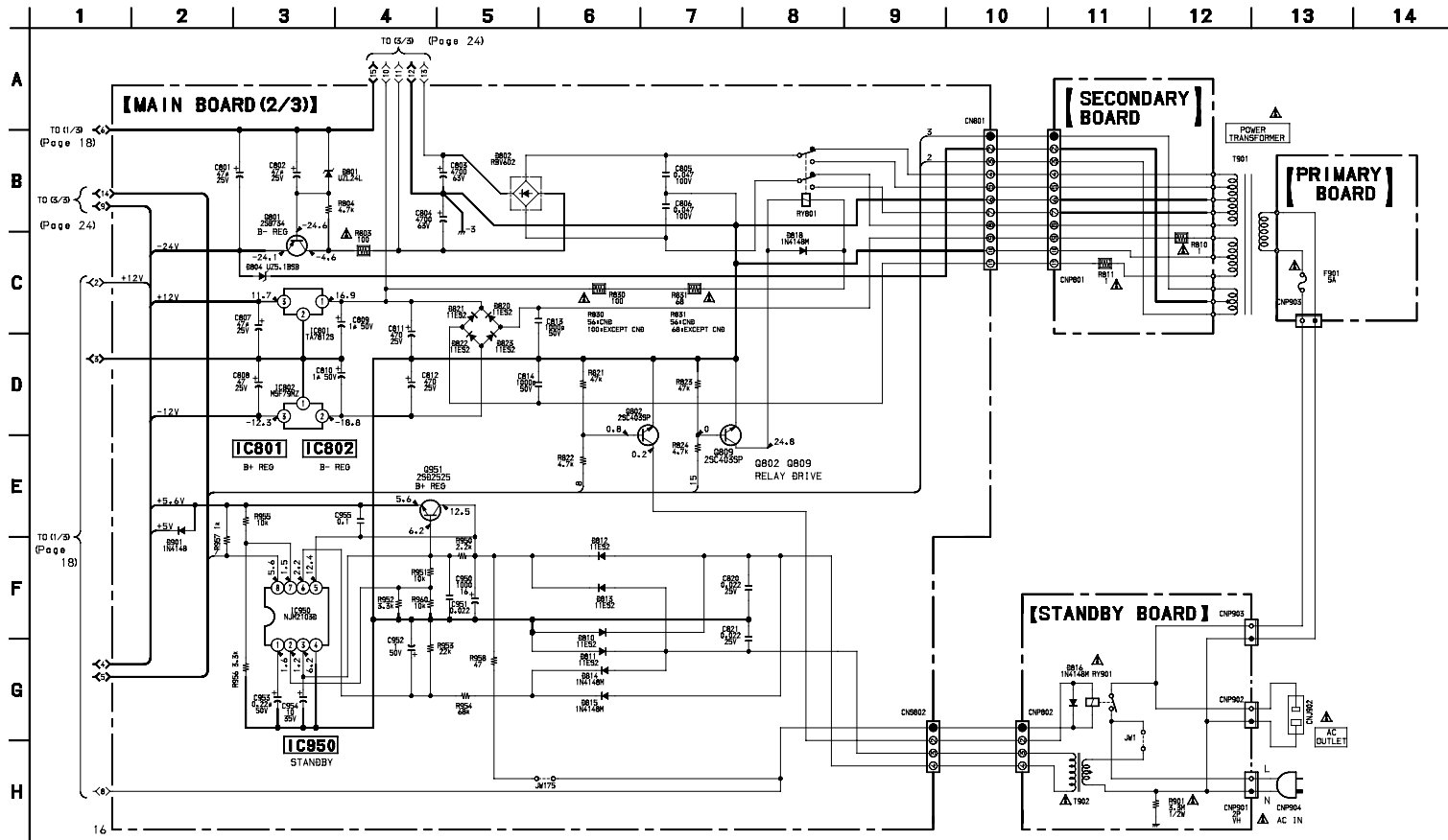
3-9. SCHEMATIC DIAGRAM — MAIN (2/3), POWER SECTION — • See page 27 for IC Block Diagrams.
