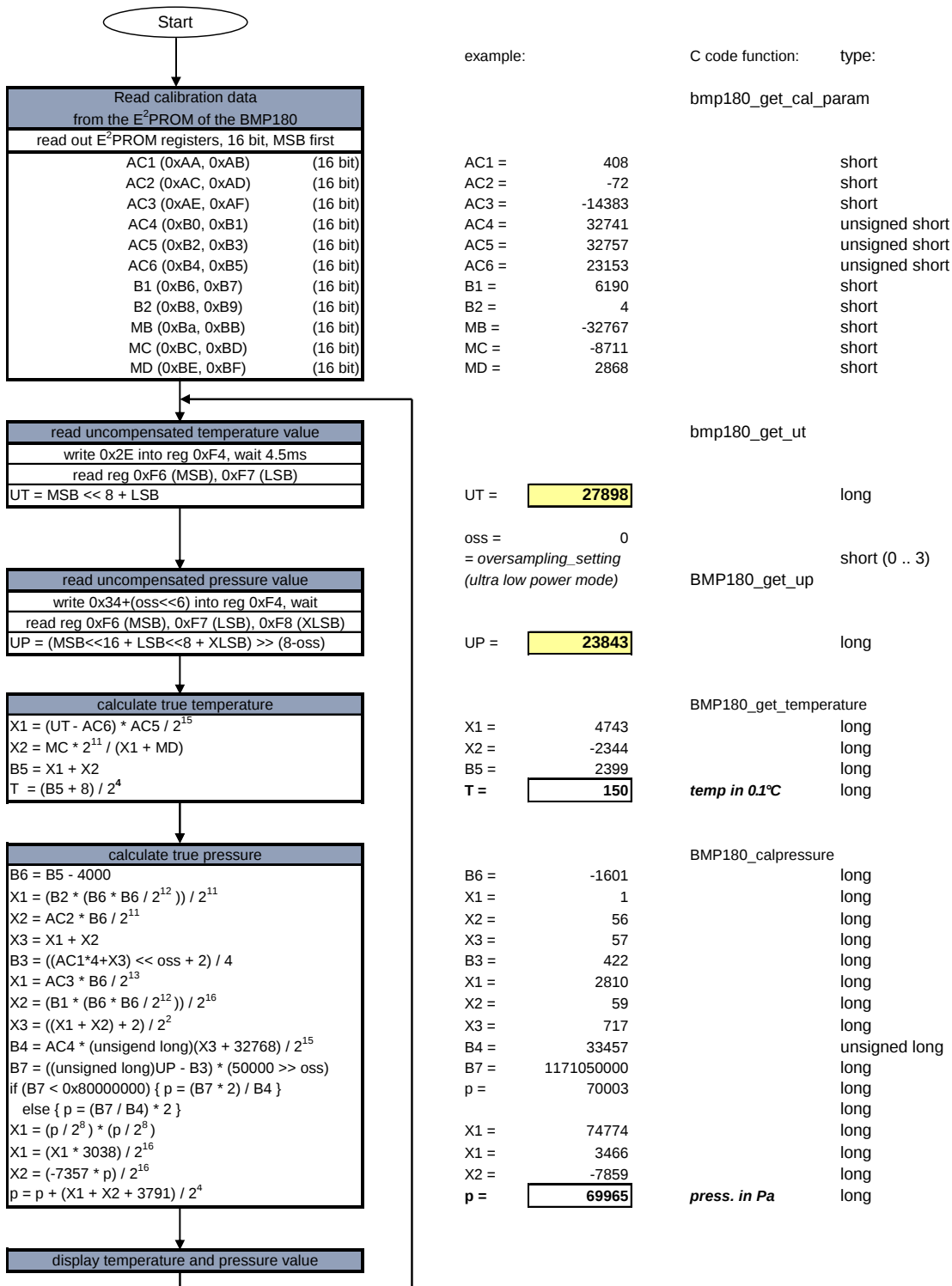
Figure 4: Algorithm for pressure and temperature measurement
