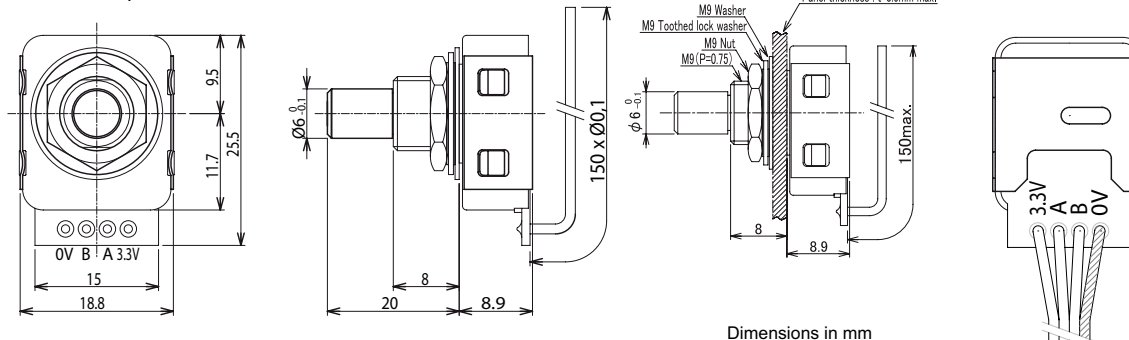
MRB without push button - V6
