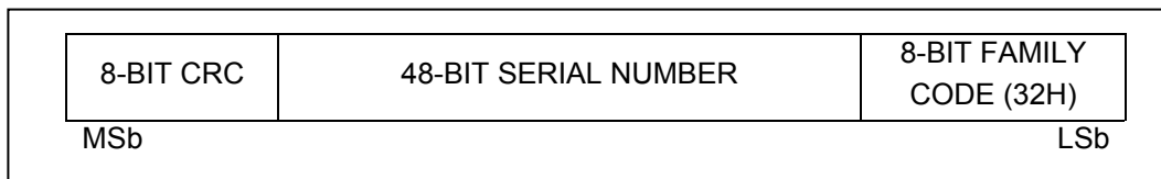
Figure 6. 1-Wire Net Address Format
