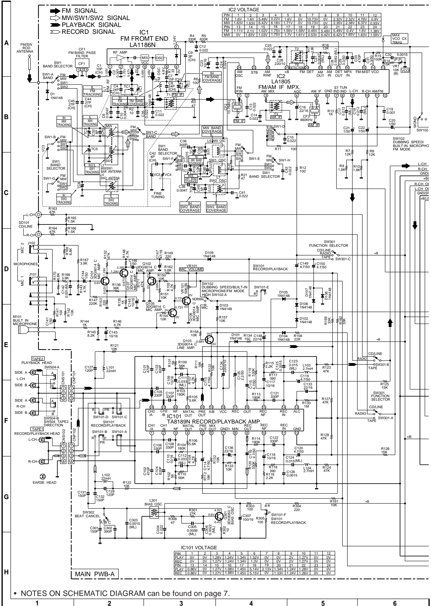
Figure 8 SCHEMATIC DIAGRAM (1/2)
