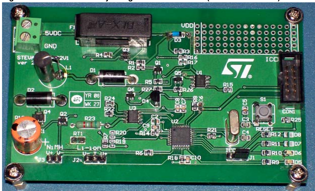
Figure 1. Universal battery charger evaluation board (STEVAL-ISB002V1)
