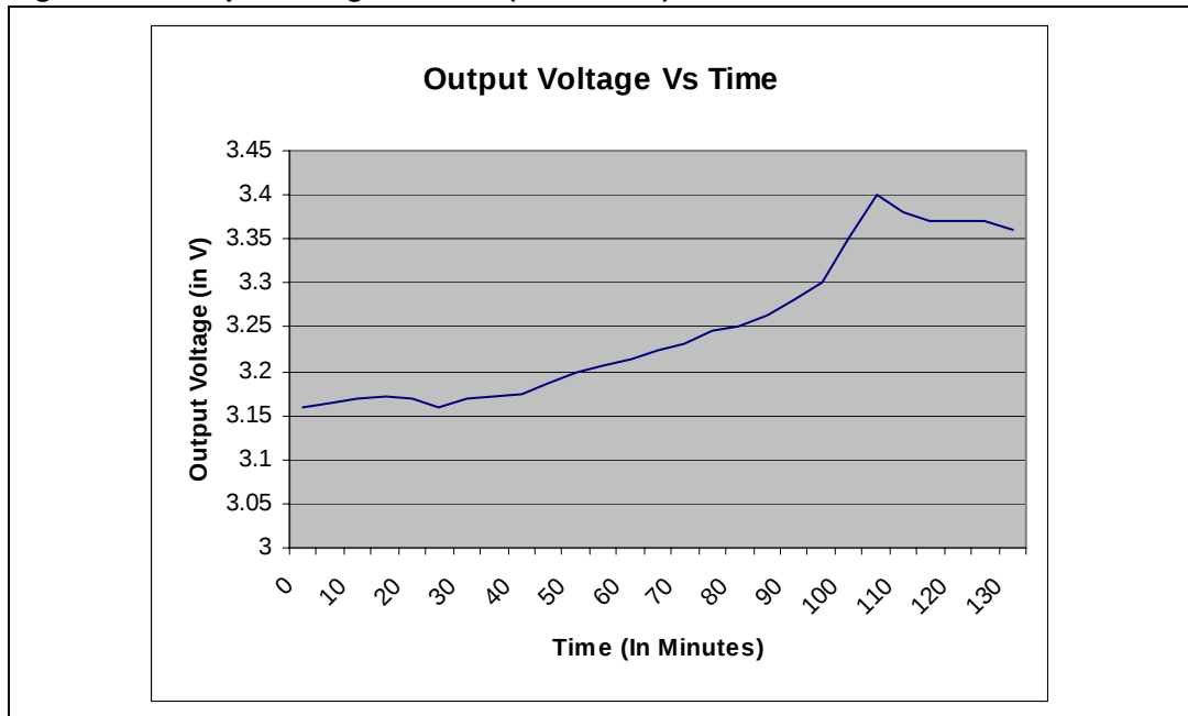
Figure 21. Output voltage vs. time (in minutes)
