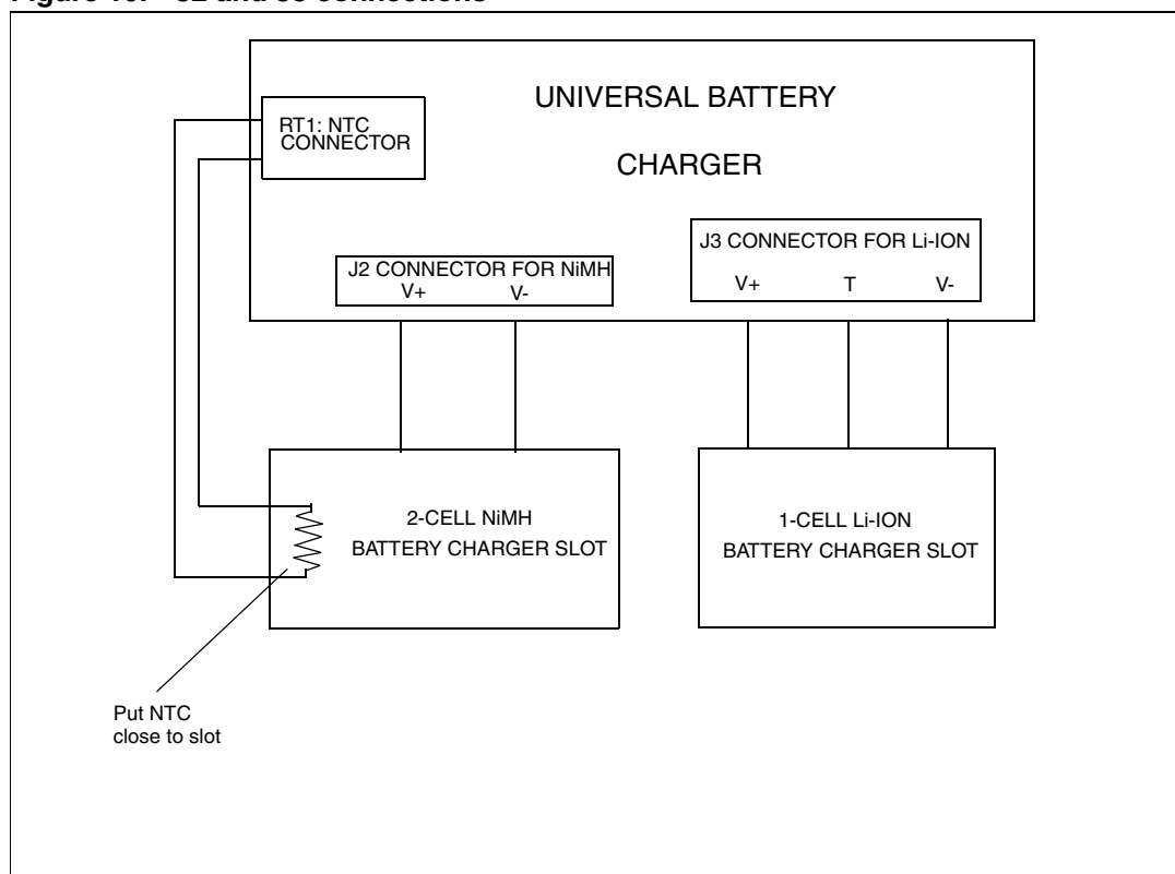
Figure 19. J2 and J3 connections
