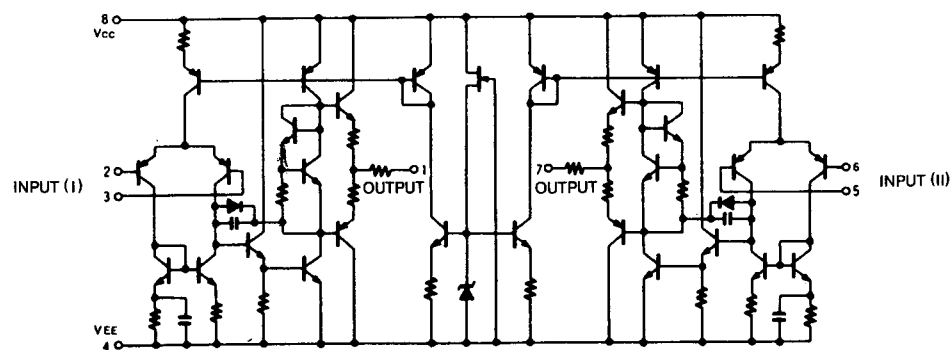
(3) NJM4558
