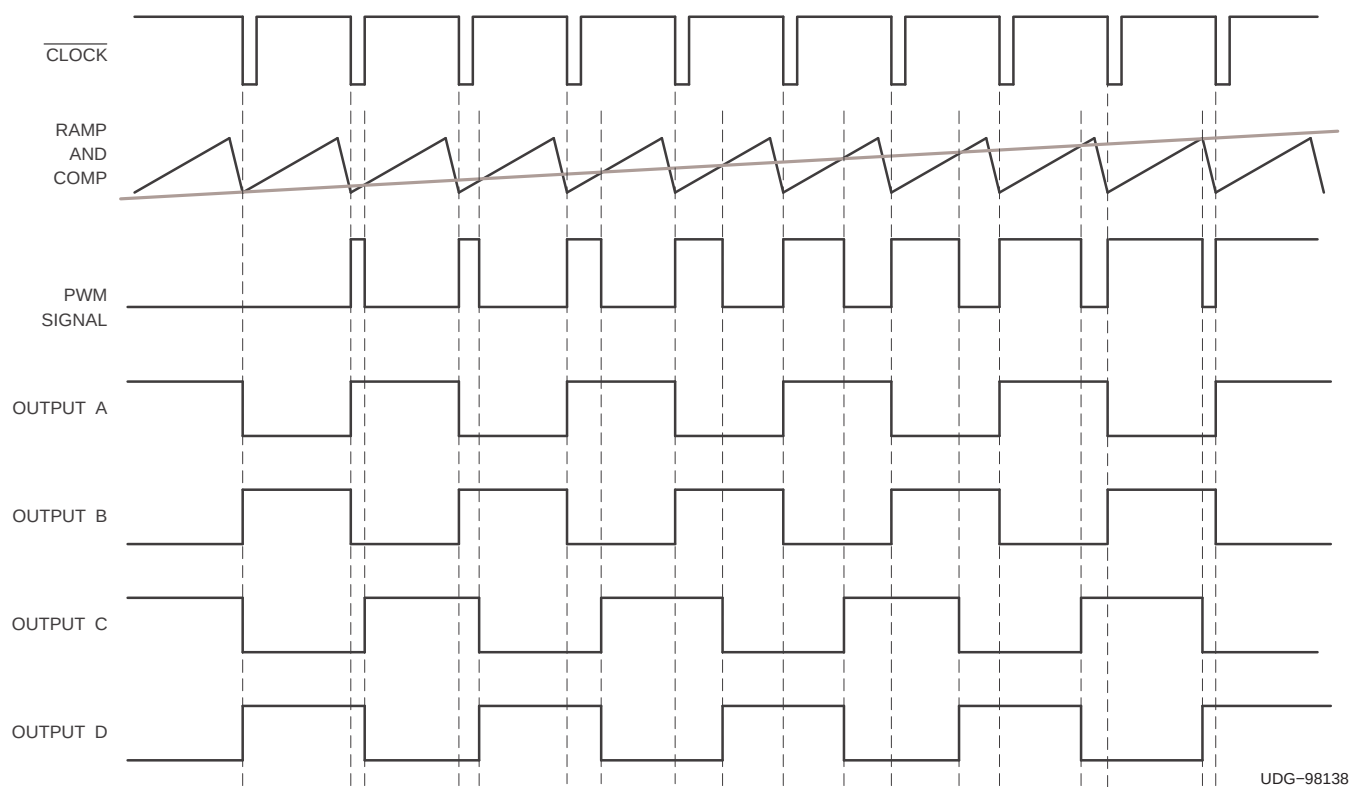
Figure 5. UCC2895-EP Timing (No Output Delay Shown)
