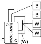
SHORT SWITCH TOP
