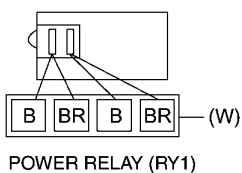
POWER RELAY (RY1)
