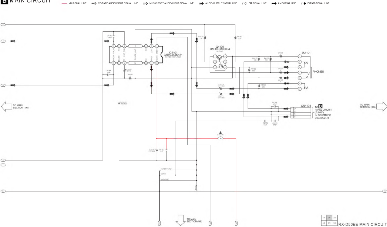
SCHEMATIC DIAGRAM - 3
