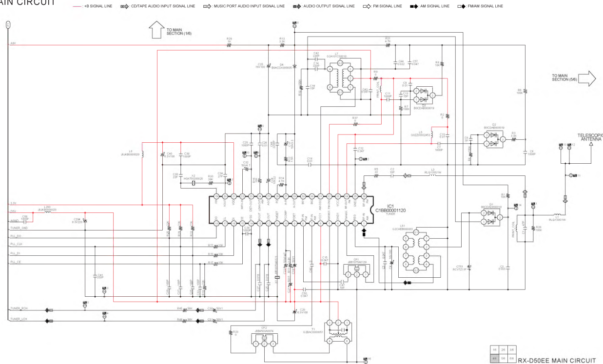
SCHEMATIC DIAGRAM - 5
