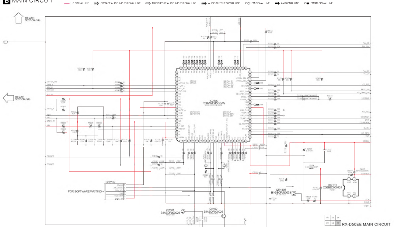
SCHEMATIC DIAGRAM - 7
