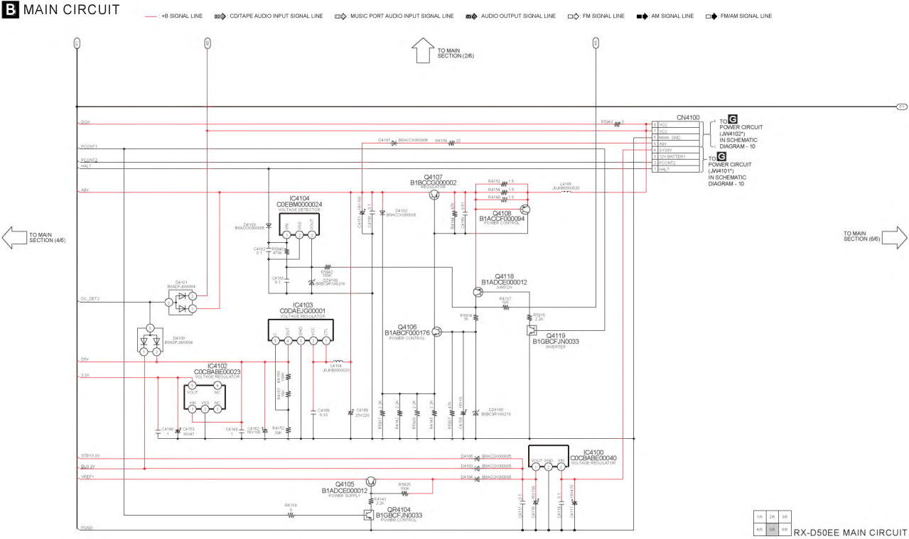
SCHEMATIC DIAGRAM - 6
