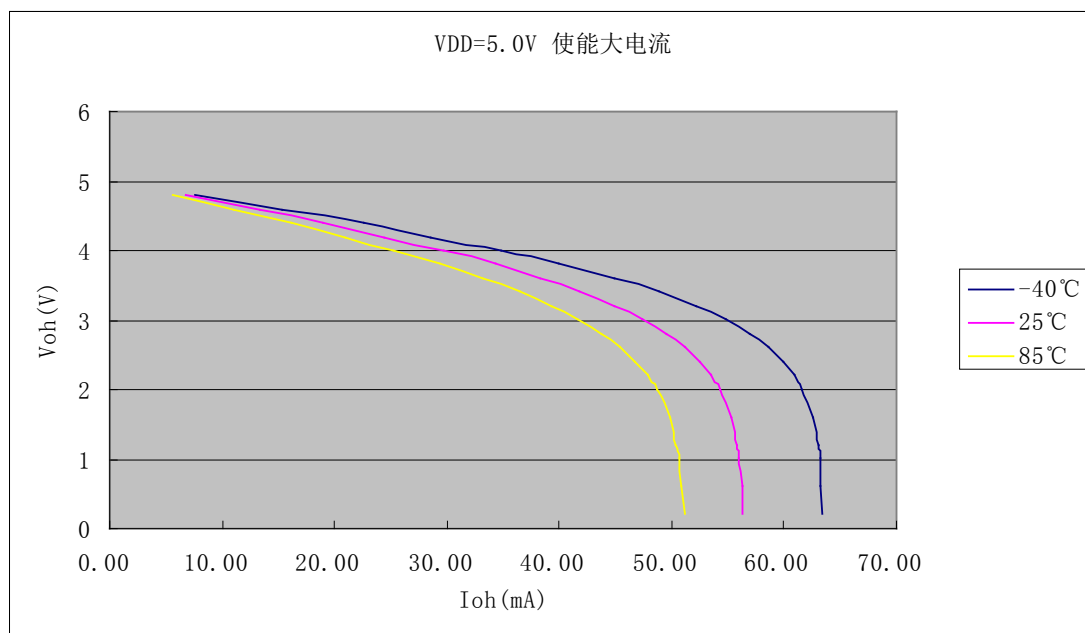
E: V_{OH} vs I_{OH} @VDD=5.0V
