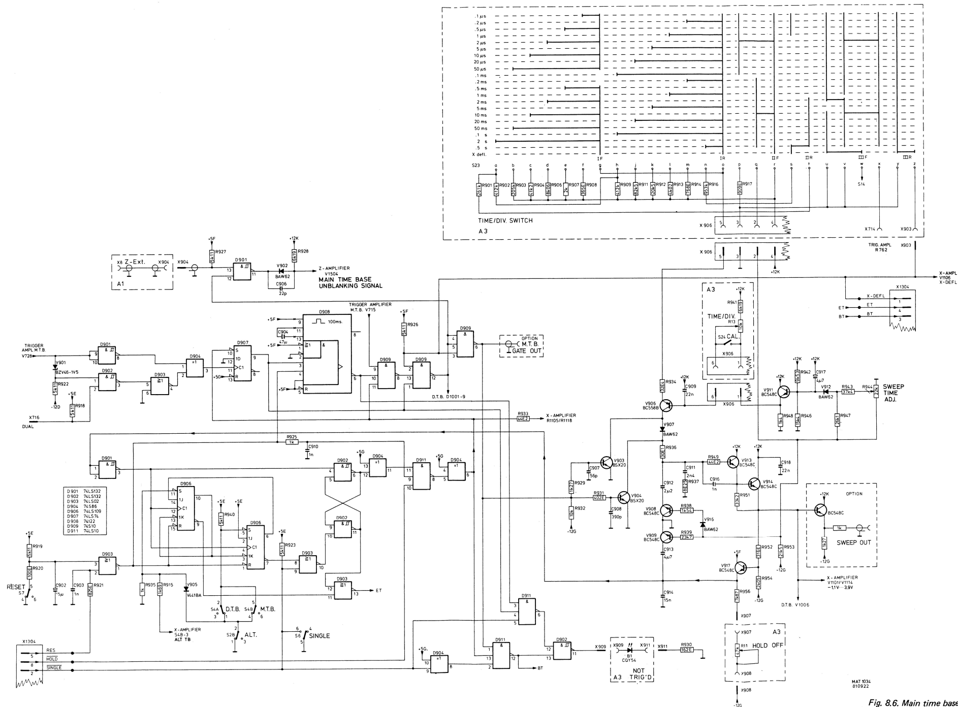
Fig. 8.6. Main time base
