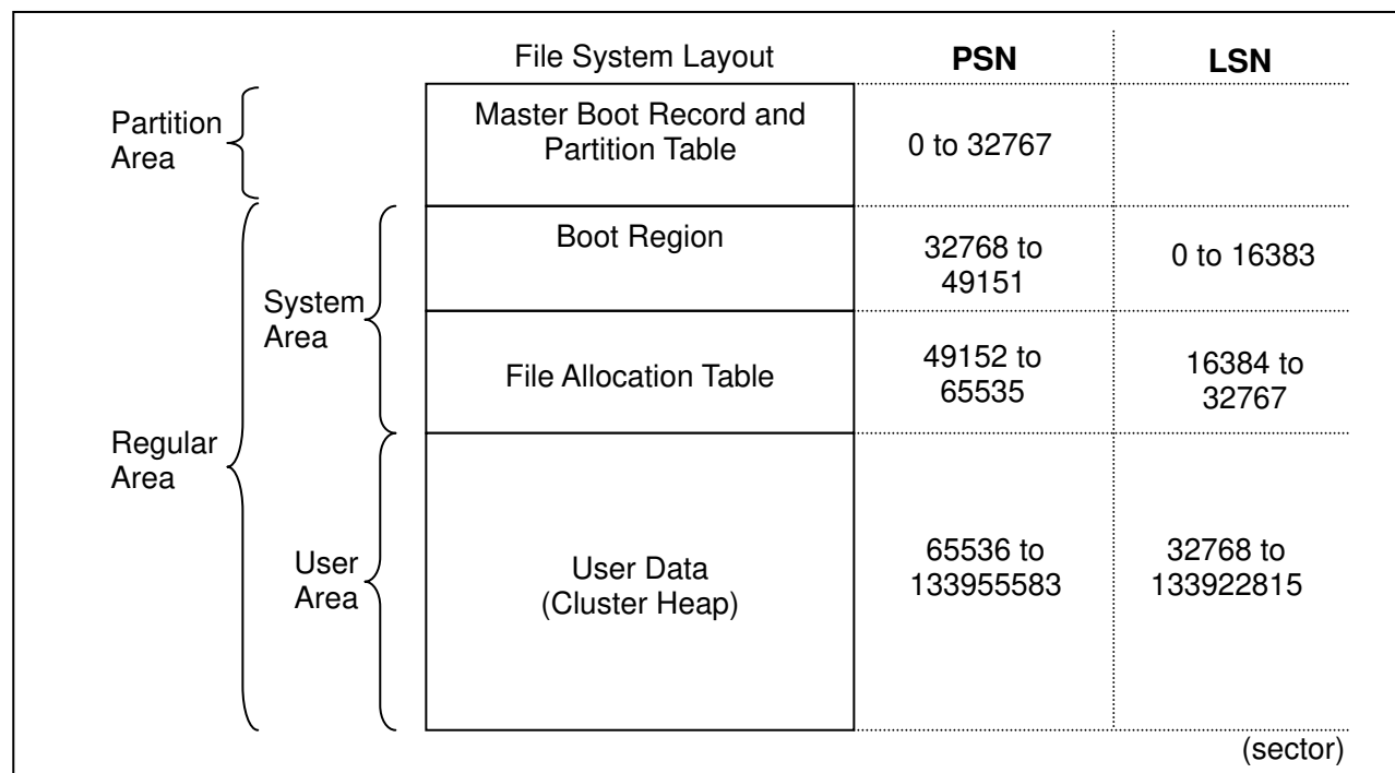
Figure 5-1 : Example of Volume Structure for Data Area
