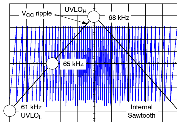
Figure 15. The V_{CC} Ripple is used to Introduce a Frequency Jittering on the Internal Oscillator Sawtooth
