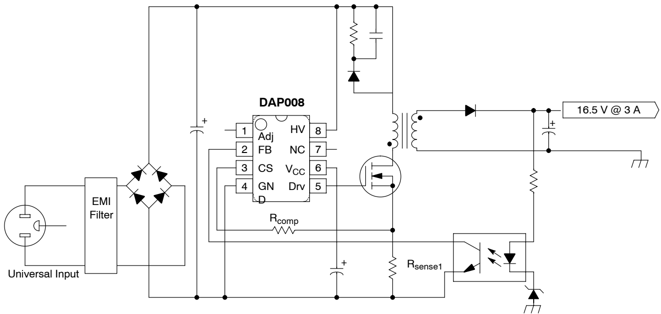
Figure 1. Typical Application
