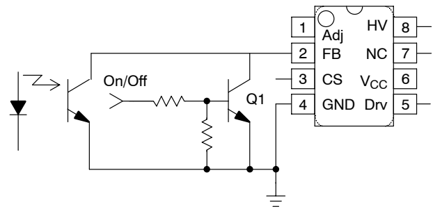
Figure 20. Another Way of Shutting Down the IC Without a Definitive Latch-Off State
