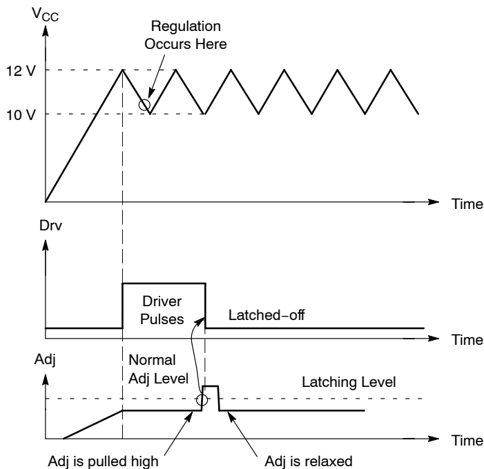
Figure 21. When V_{adj} is Pulled Above 3.2 V, DAP008 Permanently Latches-Off the Output Pulses
