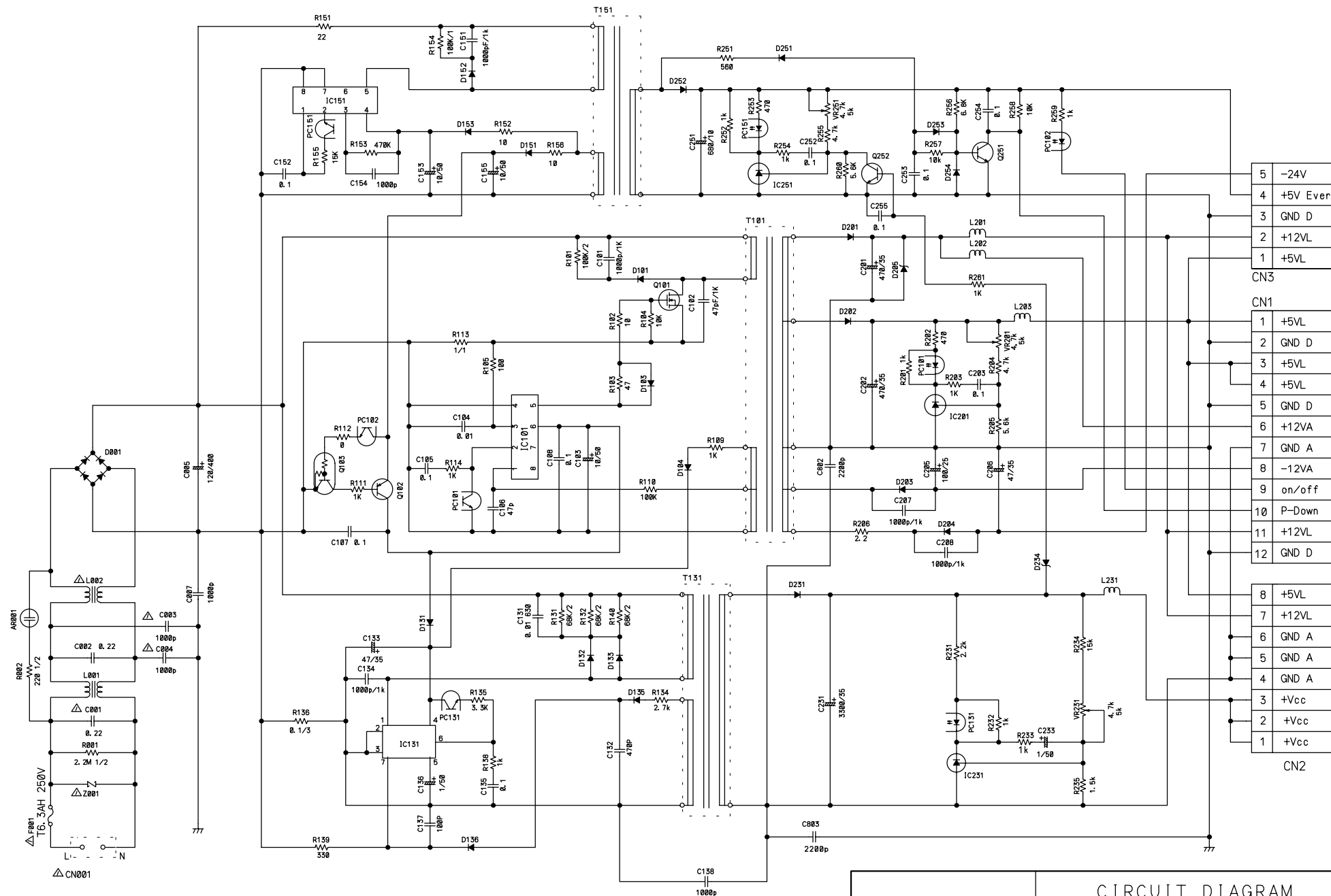
CIRCUIT DIAGRAM
