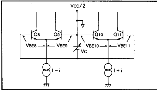
Fig. 2 Differential circuit
