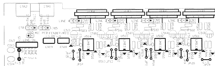
Microphone PCB Component Side
