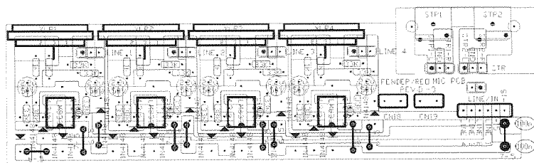
Microphone PCB Copper Side
