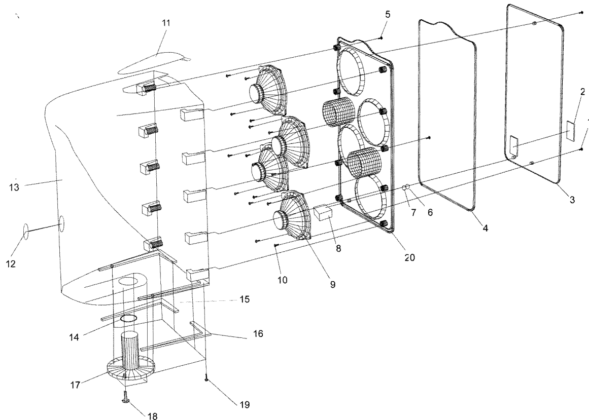
SPEAKER BOX ASSEMBLY EXPLODED VIEW
