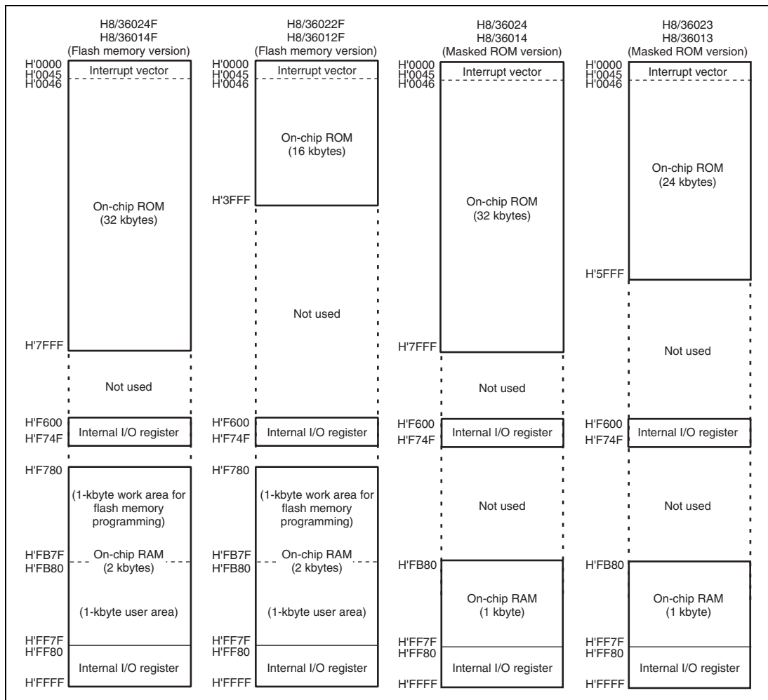
Figure 2.1 Memory Map (1)
