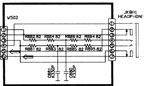
K HEADPHONE CIRCUIT
