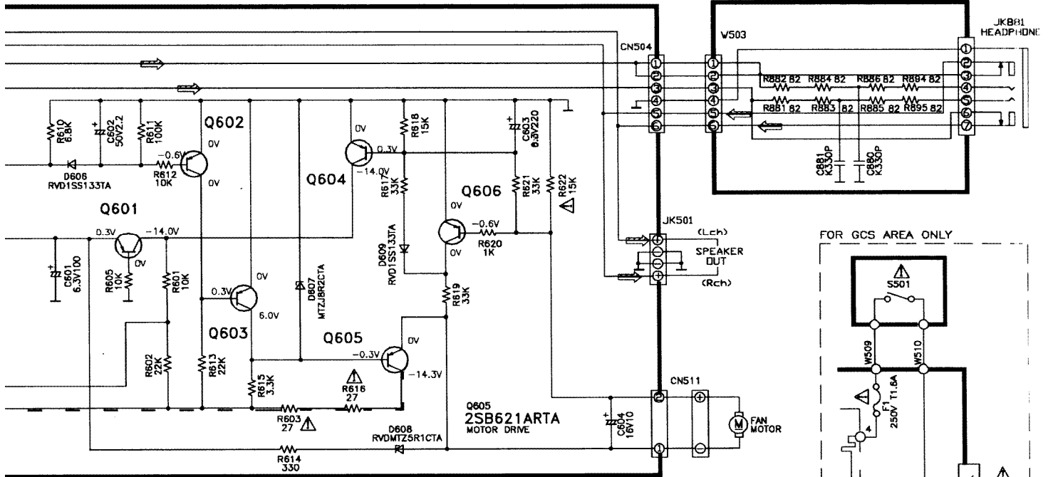
K HEADPHONE CIRCUIT
