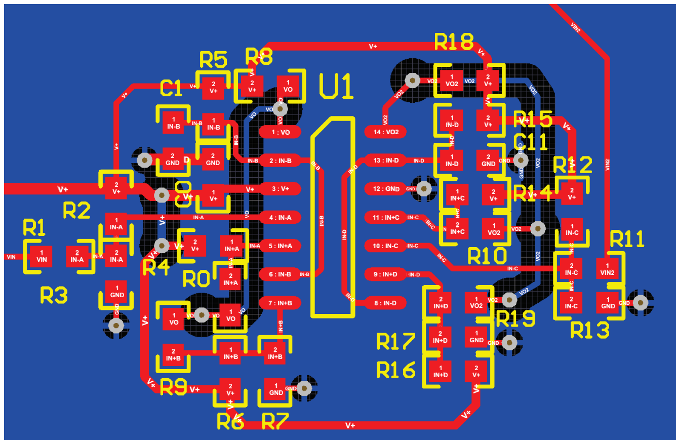
Figure 43. Layout Example
