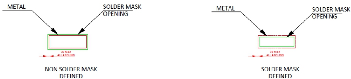
Figure 9.2 SOW8 Package Board Layout Example
