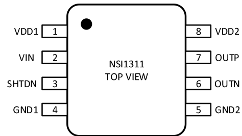
Figure 1.1 NSi1311 Package
