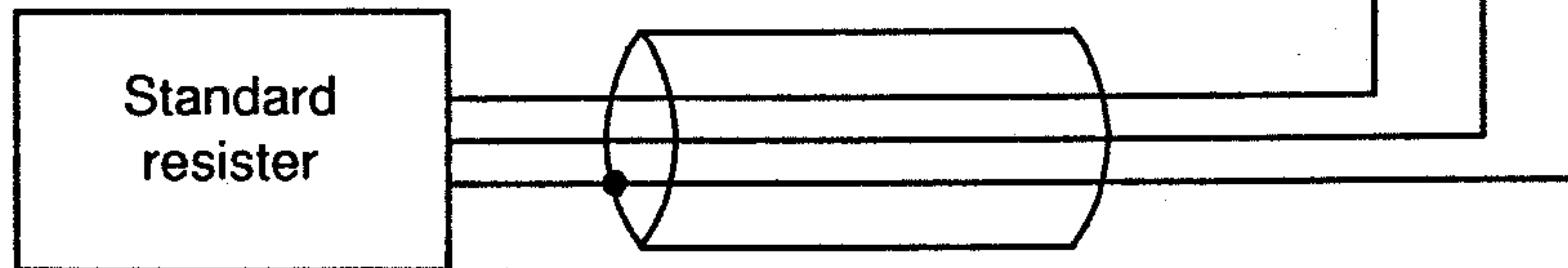
Figure 6-7 0-point Calibration of 2-wire Resistance Measurement
