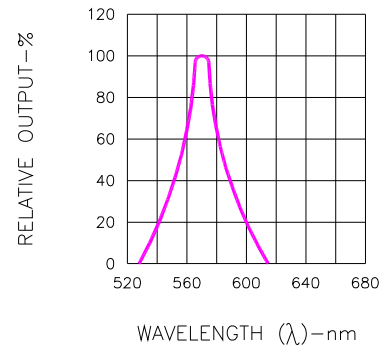
Fig.2 SPECTRAL RESPONSE
