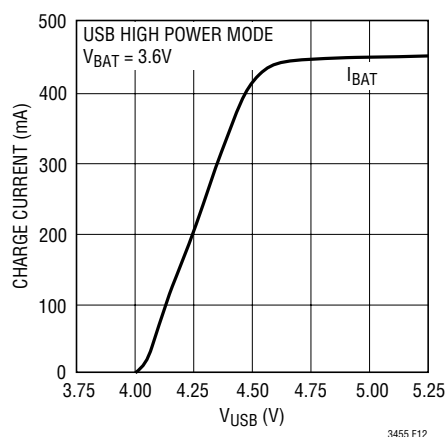
Figure 12. Charge Current vs USB Voltage
