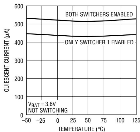
PWM Mode Quiescent Current
