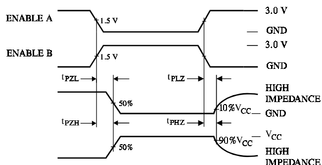
Figure 2. Switching Waveforms
