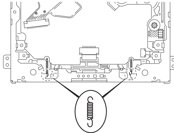
Floating spring
