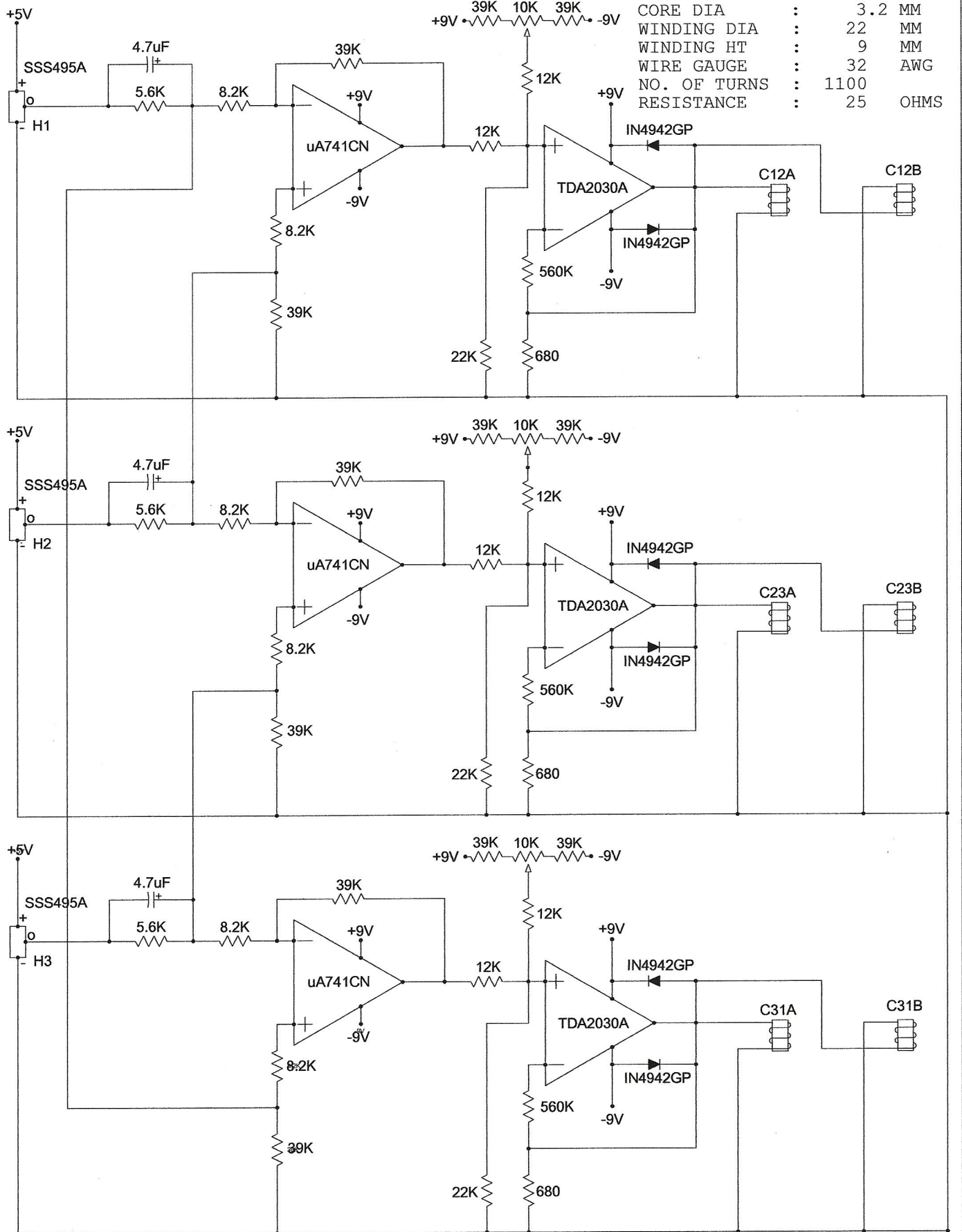
BASIC DIAGRAM FOR REPULSIVE ELECTROMAGNETIC LEVITATOR, 6 FIELD COIL CONFIGURATION
