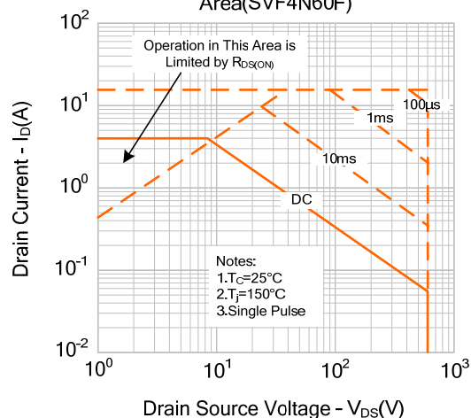
Figure 9-2. Max. Safe Operating Area(SVF4N60F)
