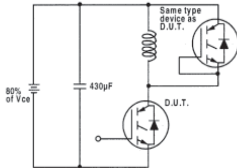
Fig. 18a - Test Circuit for Measurement of I_{LM} , E_{on} , E_{off}(\text{diode}) , t_{rr} , Q_{rr} , I_{rr} , t_{d(on)} , t_r , t_{d(off)} , t_i
