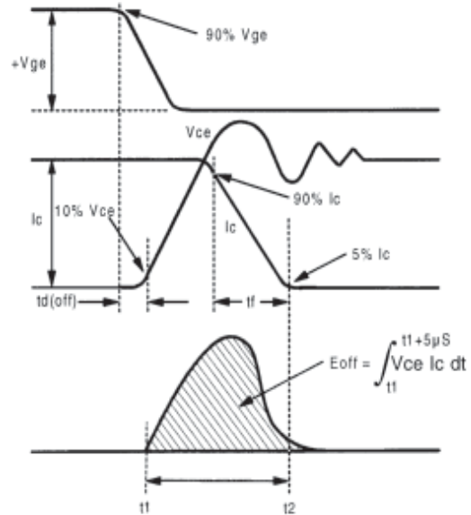
Fig. 18b - Test Waveforms for Circuit of Fig. 18a, Defining E_{off} , t_{d(off)} , t_i
