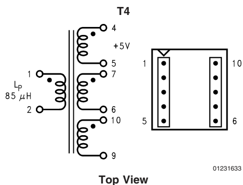
FIGURE 18. Coilcraft Q4344-B
