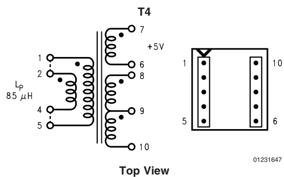
FIGURE 32. Schott 67140930
