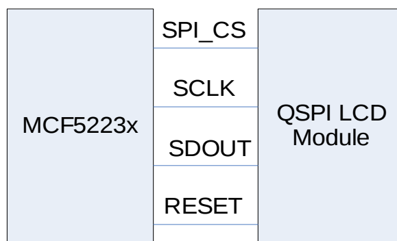
Figure 6. QSPI LCD Interface Connection with ColdFire
