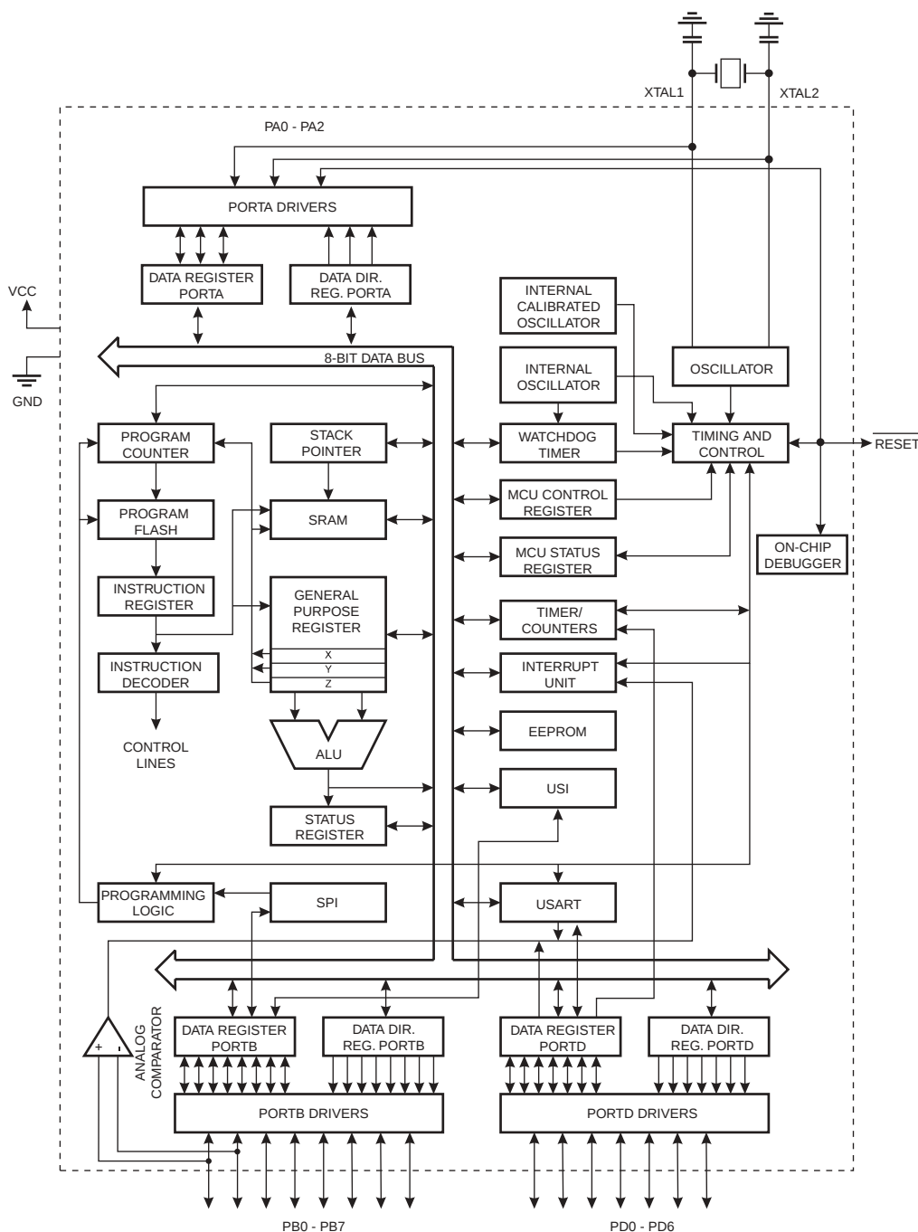
Figure 2. Block Diagram
